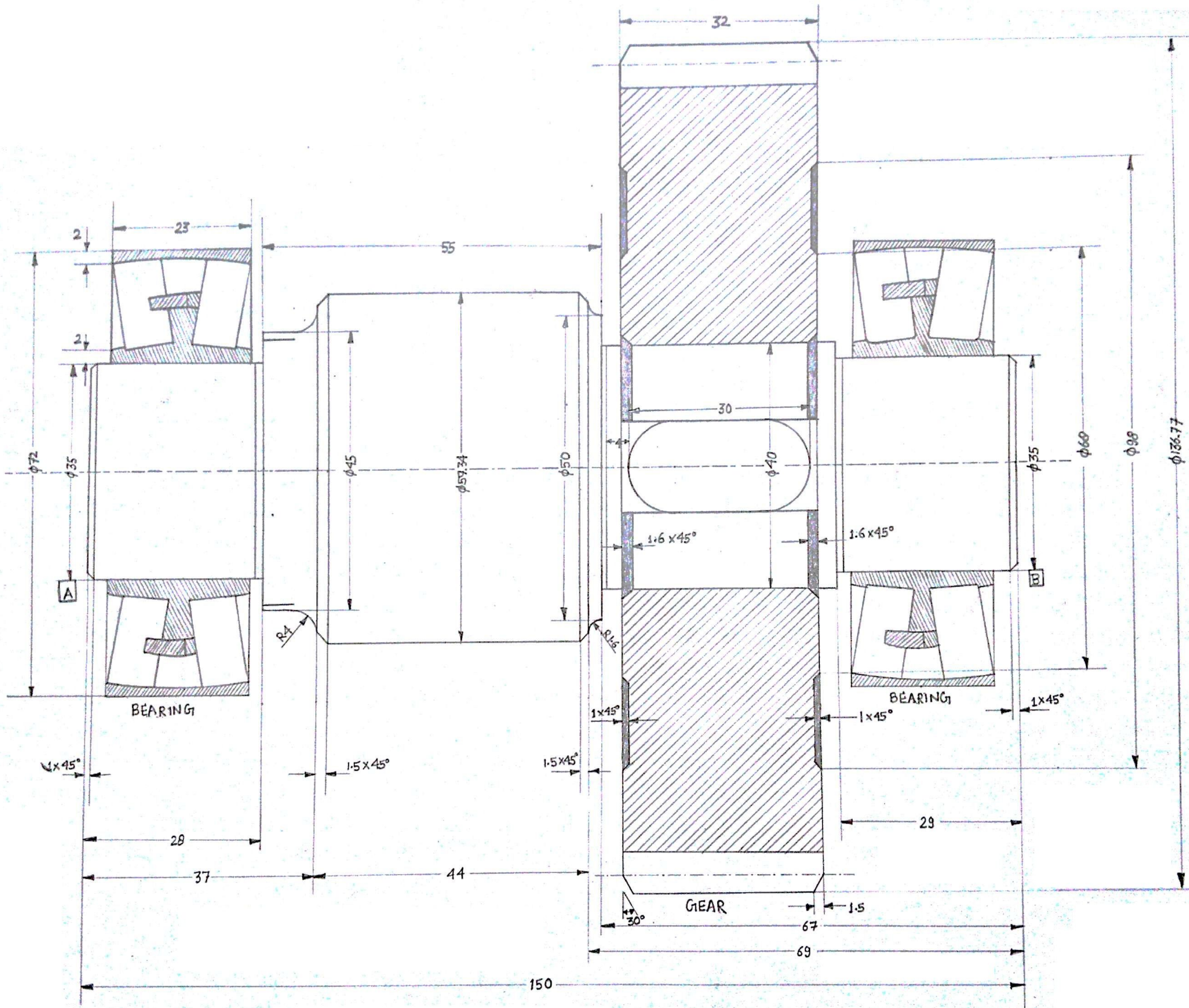
PINION WITH INTEGRAL SHAFT
